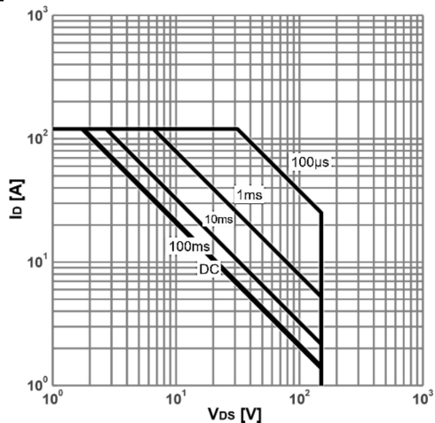
Figure 1. Power dissipation
